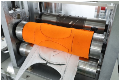
切刀轮装置 Cutting roller
