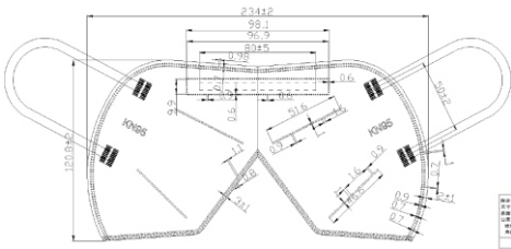
压花轮图案可根据客户需求订制 Teeth roller patterns according to customized design
