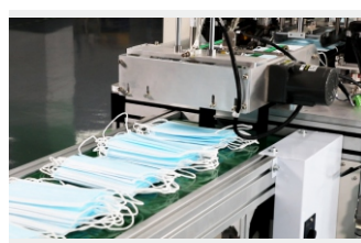
收料输送带机构 Collector conveyor mechanism
