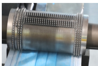
压花轮机构 Compressing mechanism
